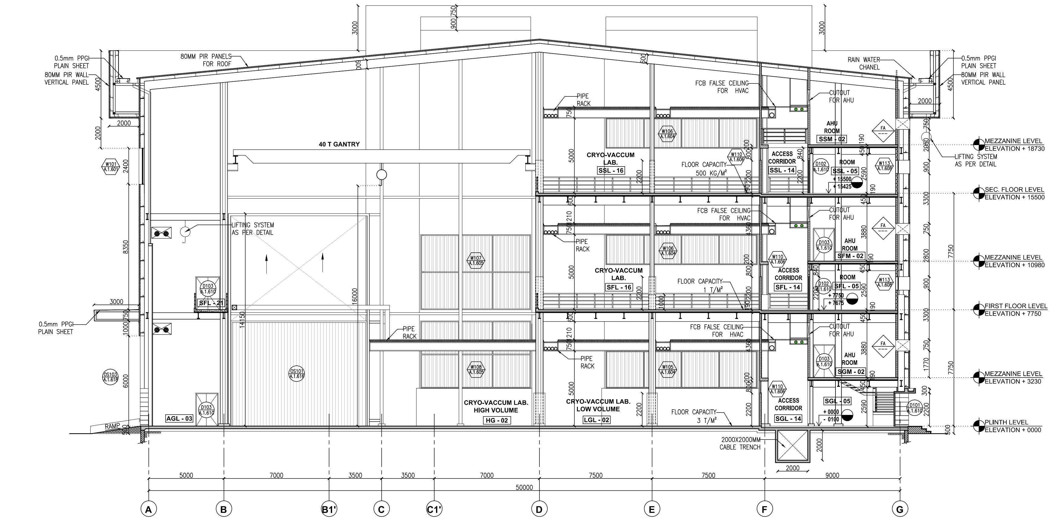
1 SECTION SCALE 1:150
